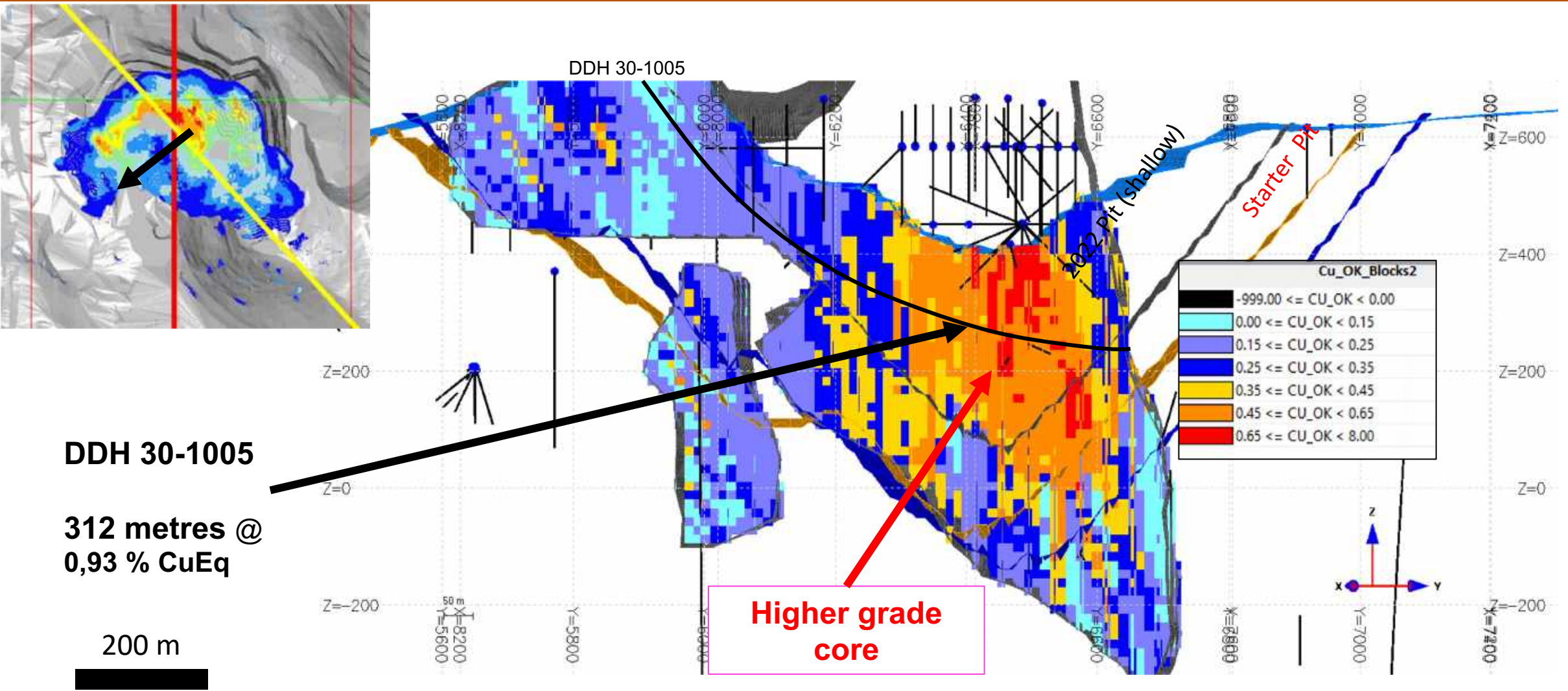
Block model in vertical section looking SW
