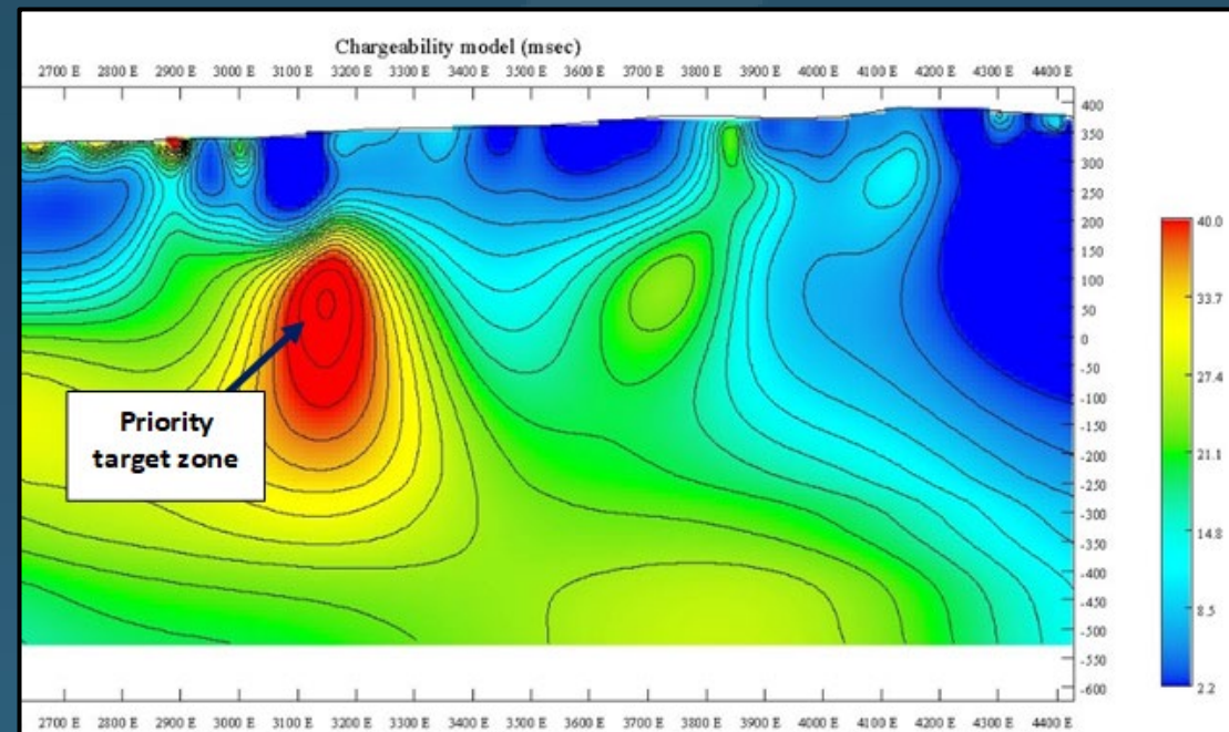
Figure 1 - Chargeability model of IP survey line 6,452,000N showing the location of the sulphide target zone at North Callisto (see map on previous slide for line location)
