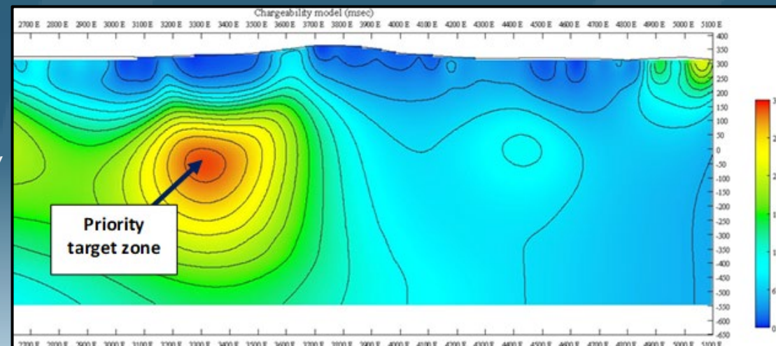
Figure 2 - Chargeability model of IP survey line 6,453,200N showing the location of the sulphide target zone at North Callisto (see map on previous slide for line location)
