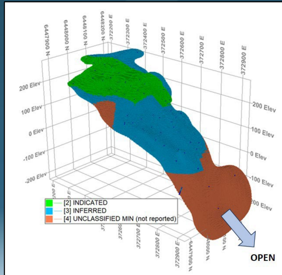
Callisto resource classification showing mineralisation continuing at depth
