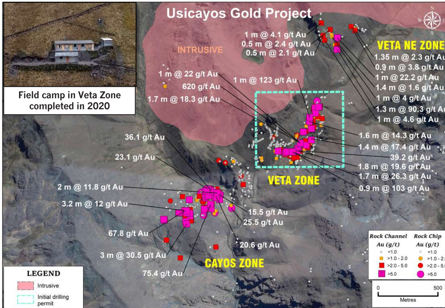
Top ten select channel and rock samples for the Veta, Veta NE and Cayos Zones October 27, 2020
